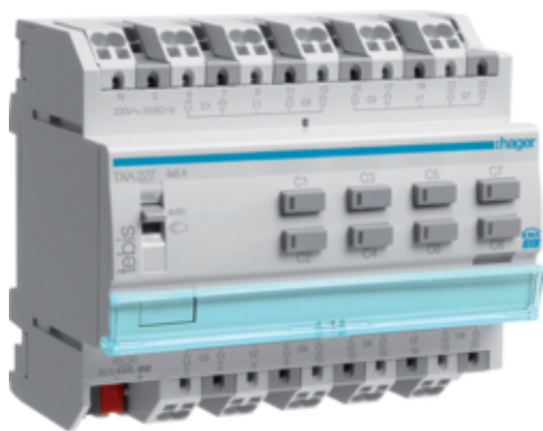
Output device for 8 shutters 230V~
