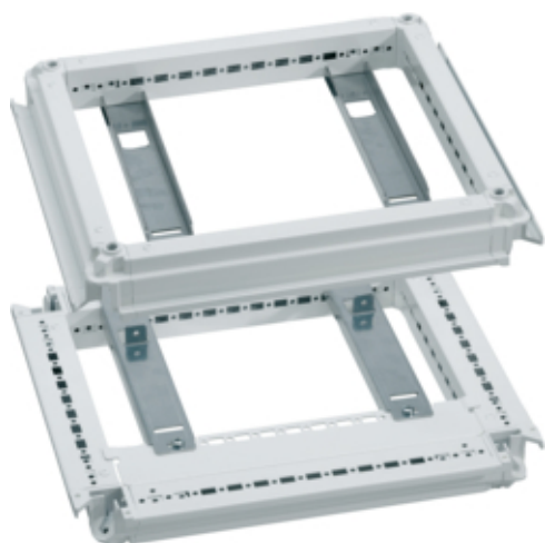
Top and bottom, Quadro.Plus, 700x800 mm
