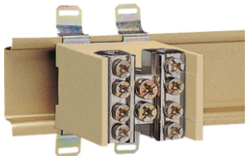
Main line branch terminal, 1 p., 1x35mm 2 - 4x25mm 2
