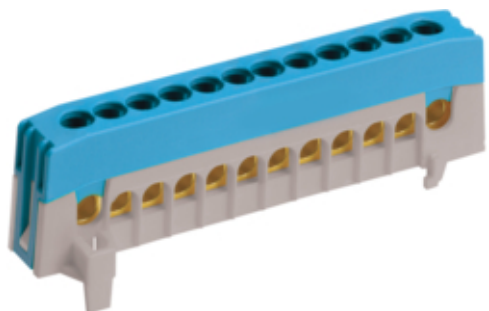
Brass-Terminal, 12x16mm 2 , IP20, Color: blue
