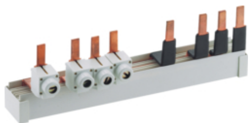
Insulated busbar HI63/125
