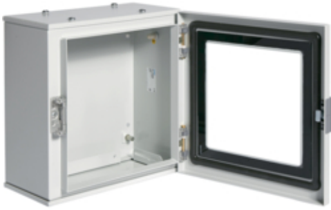
Steel enclosure, Orion.Plus, glazed door 300x300x160 mm
