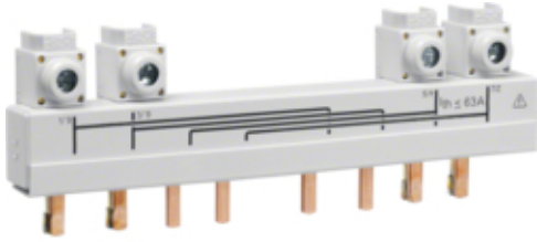
Insulated busbar 4P change over 20-40A HIM402 HIM404
