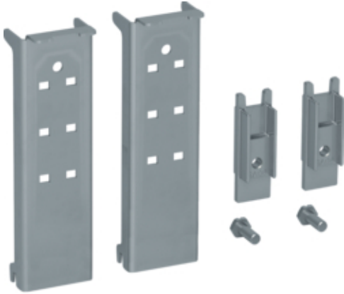
Adj. rail holder, Univers, CL1, D275 mm RAL7035
